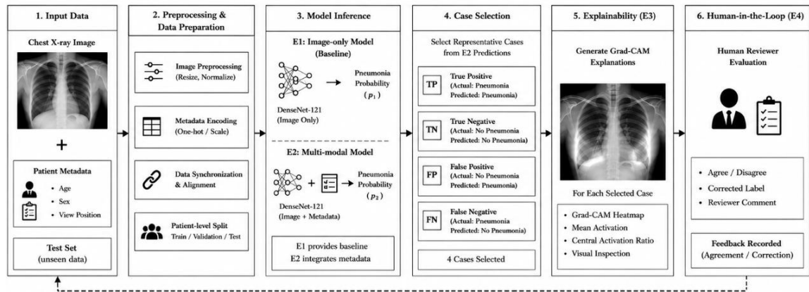
Figure 3.4.1: Framework pipeline workflow
